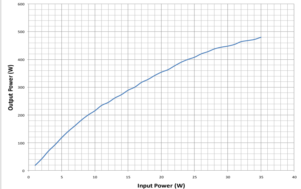
Typical O/P Power KL703 28.000MHz
